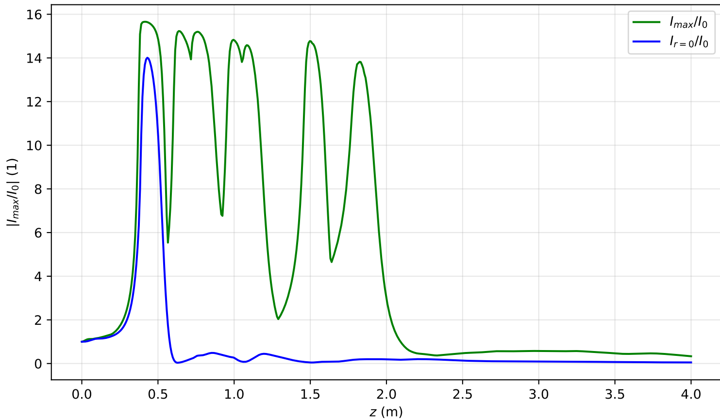
I_{max}(x=0, y=0, z)/I_0 , P_{in}=7.1P_{cr} , noisy input, artificial time
